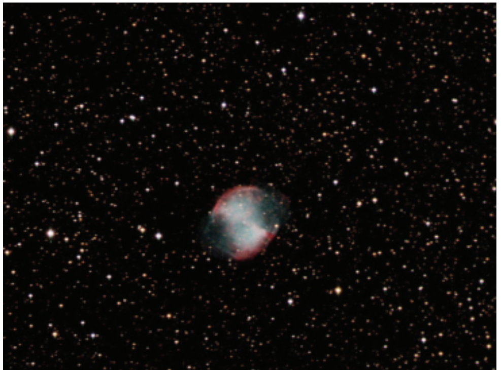
Image 8 - Shows the Dumbbell Nebula (M27) taken with a SBIG ST-10 CCD camera with the 16-day old Moon looming overhead. The exposure was 5 minutes each through red, green and blue filters.
